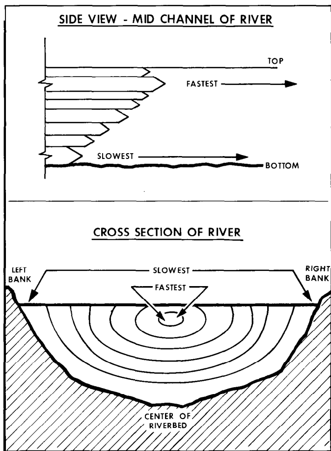
Figure 23-12. Laminar Flow.
