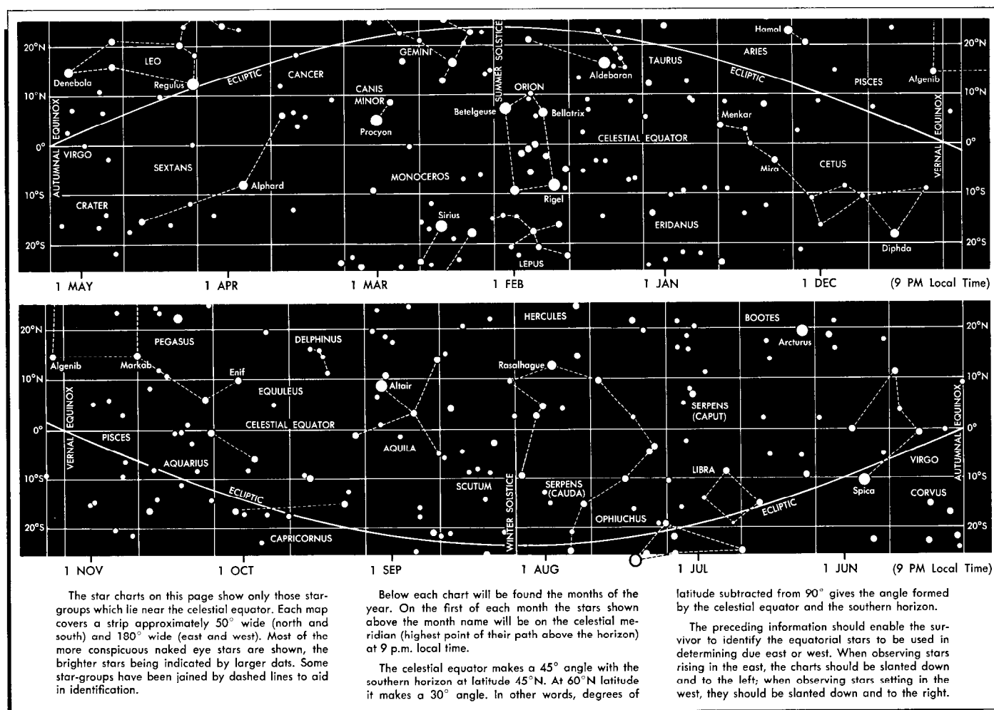
Figure 20-86. Charts of Equatorial Stars.
