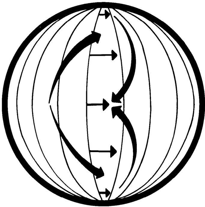
Figure 9-6. Coriolis Effect.
