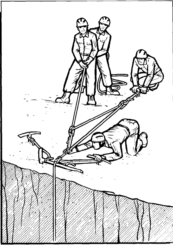
Figure 22-96. Two-Pulley System.
