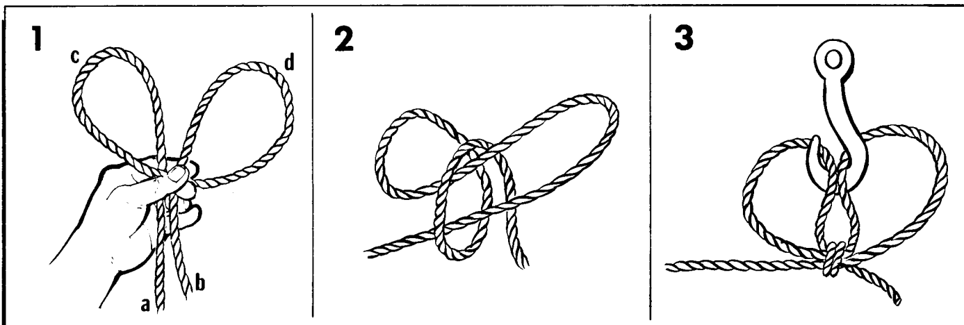
Figure 17-54. Catspaw.
