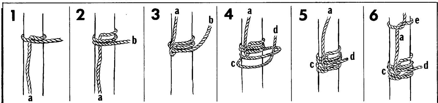
Figure 17-52. Rolling Hitch.
