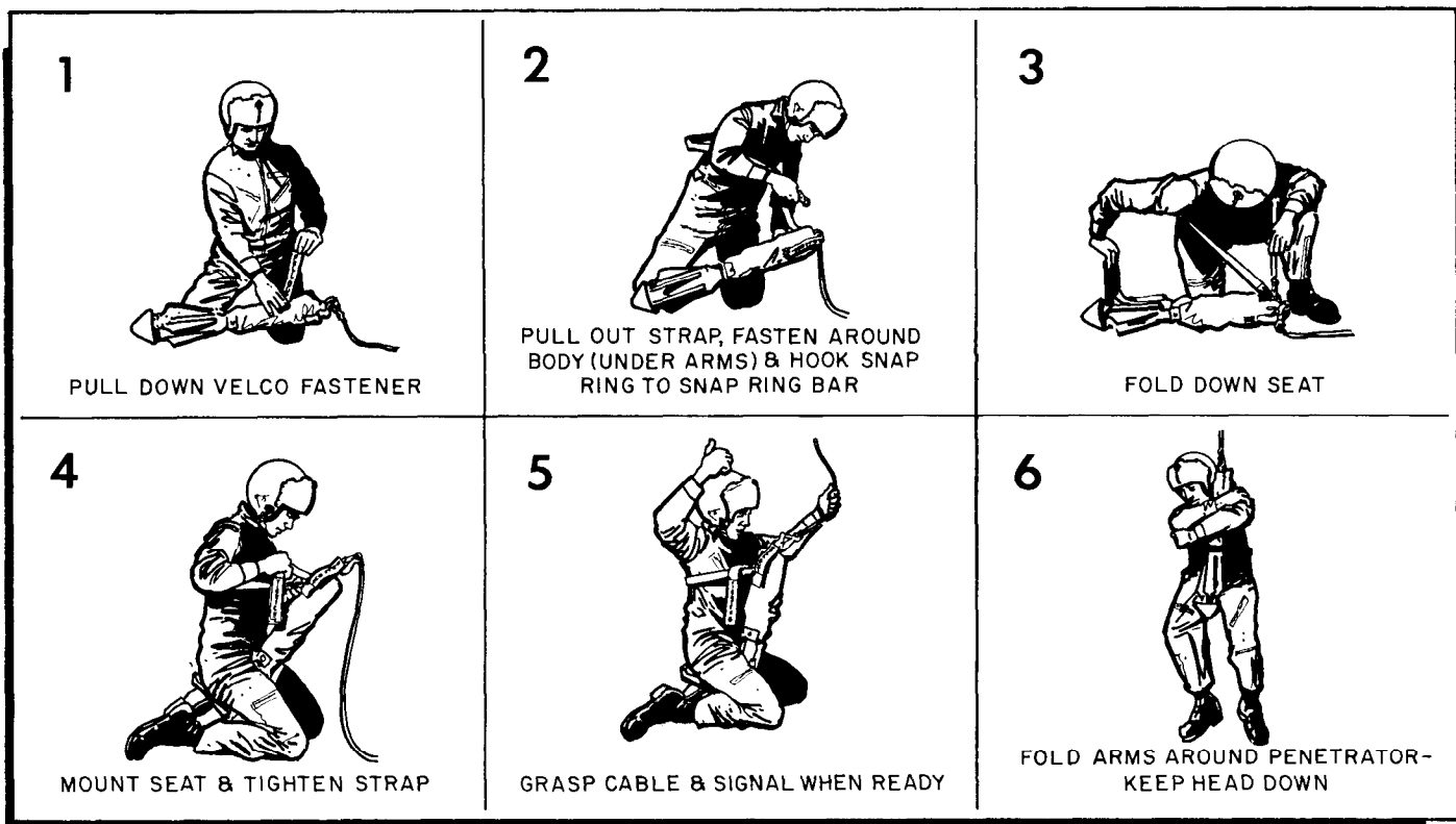
Figure 25-5. Forest Penetrator.
