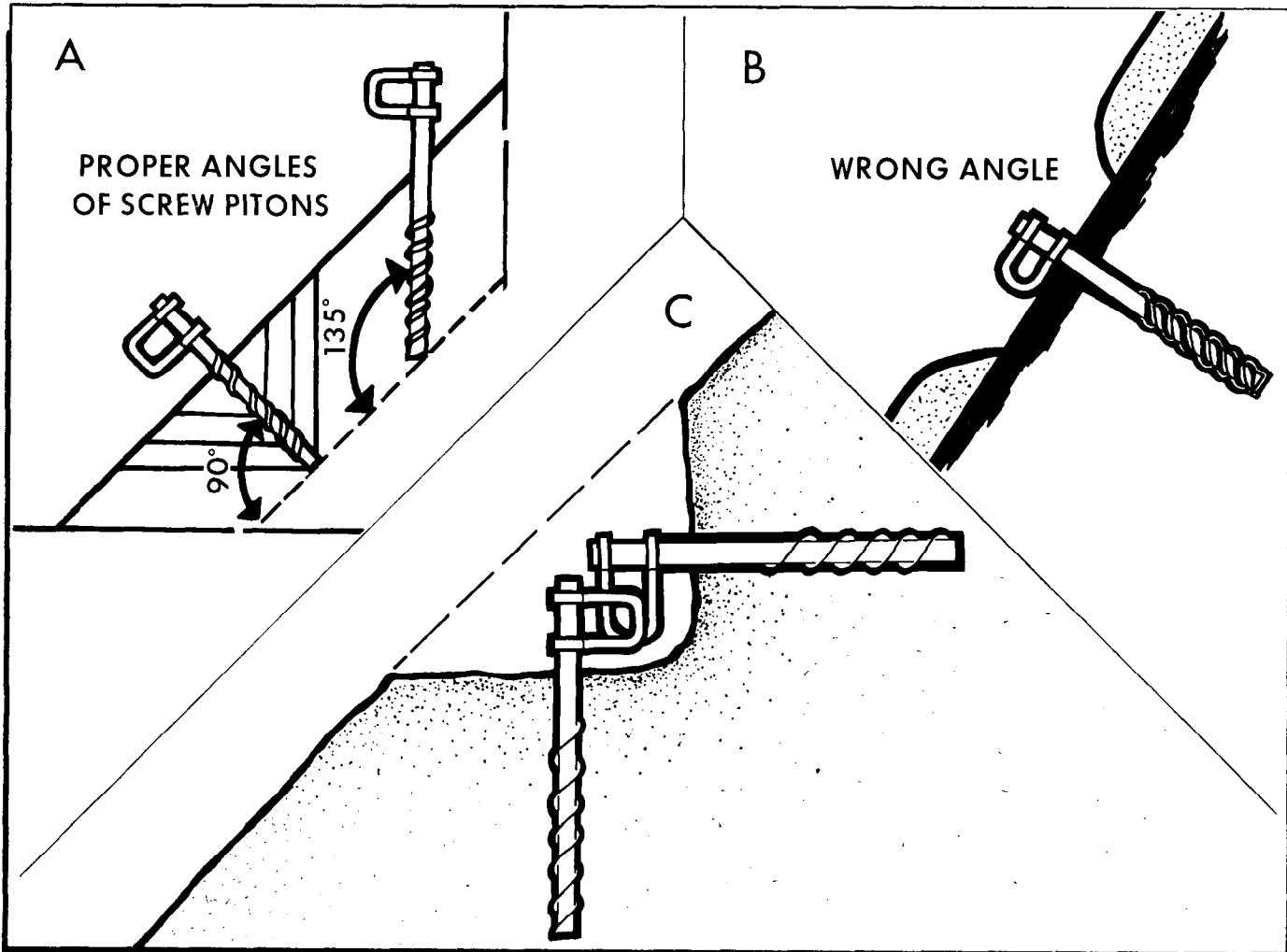
Figure 22-65. Placement of Ice Screw and Piton.
