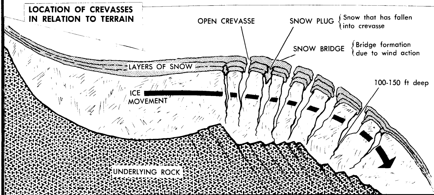
Figure 22-68. Typical Glacier Construction.
