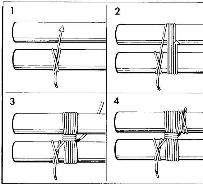
Figure 17-60. Shear Lash.
