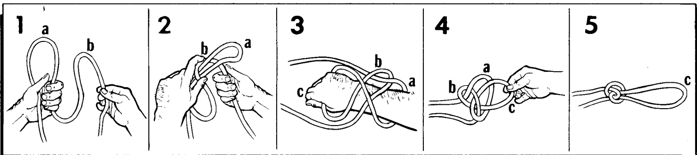
Figure 17-46. Harness Hitch.
