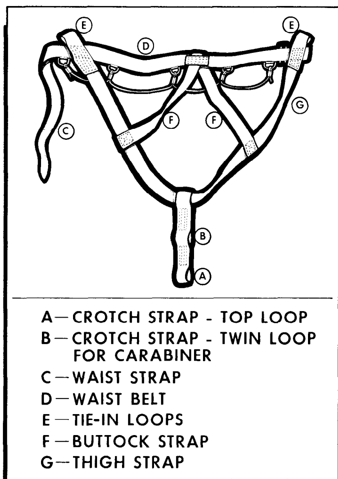
Figure 22-13. Sit Harness.
