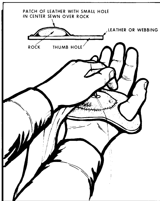
Figure 17-19. Palm Thimble.
