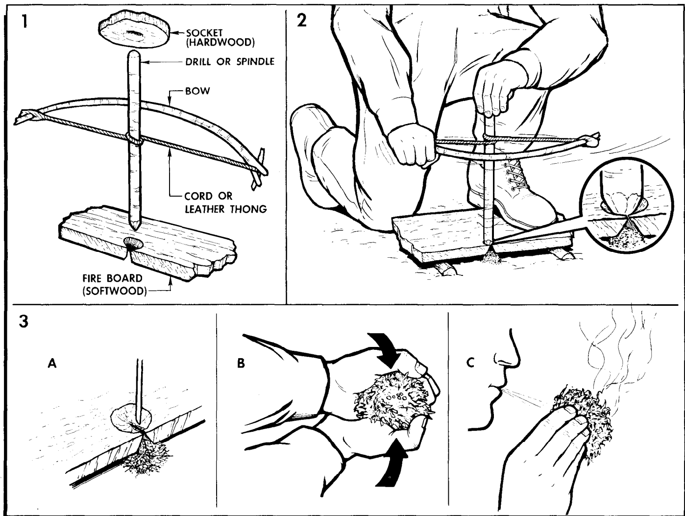
Figure 16-9. Bow and Drill.
