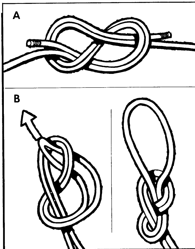
Figure 22-6. Figure-Eight Loop.
