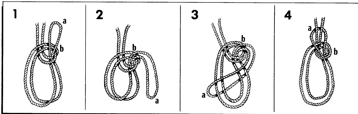
Figure 17-43. Bowline on a Bight.
