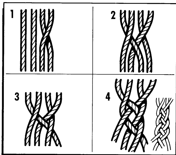
Figure 17-65. Four-Strand Braid.
