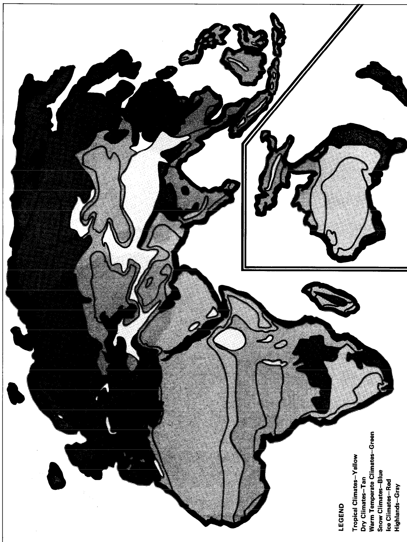
Figure 11-1. Köppen-Geiger System. (cont)
