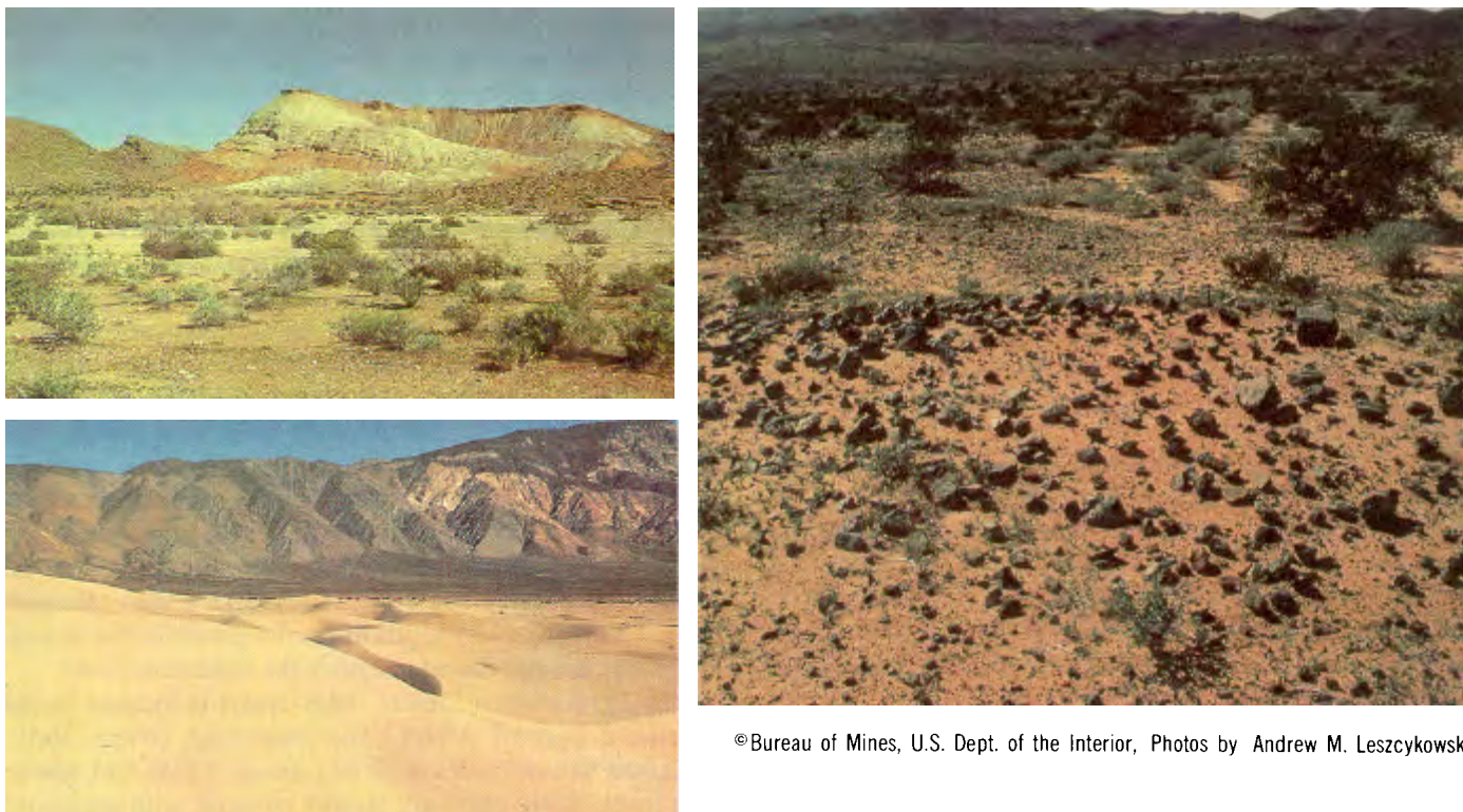
Figure 11-15. Composite of American Deserts.
