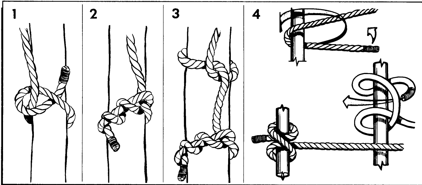
Figure 17-47. Half Hitch, Timber Hitch, and Clove Hitch.
