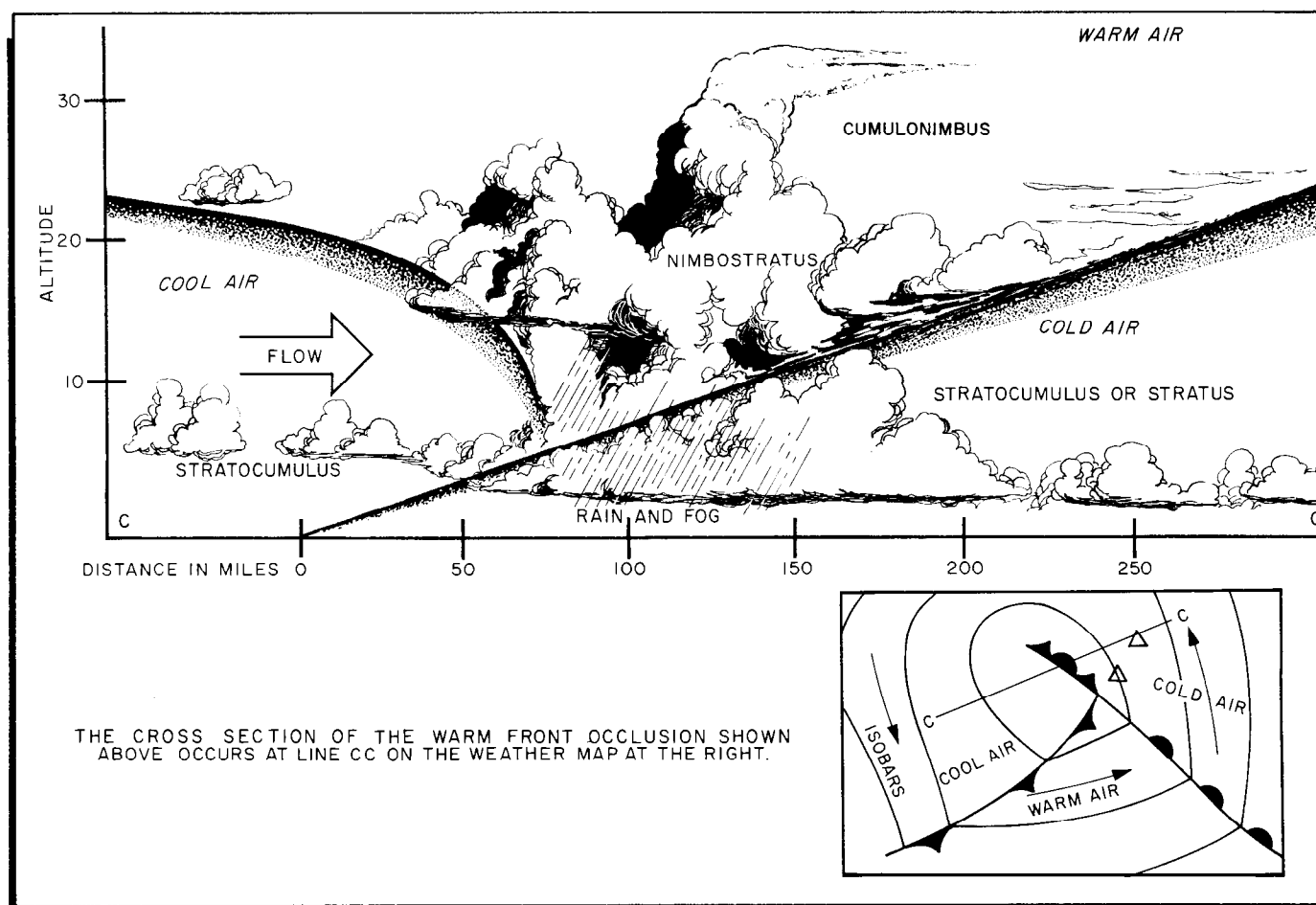
Figure 9-11. A Warm-Front Occlusion.
