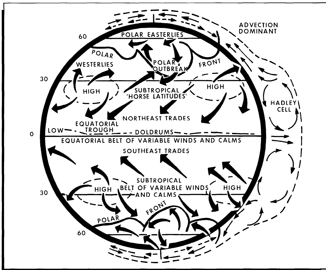
Figure 9-7. Atmosphere Circulation.
