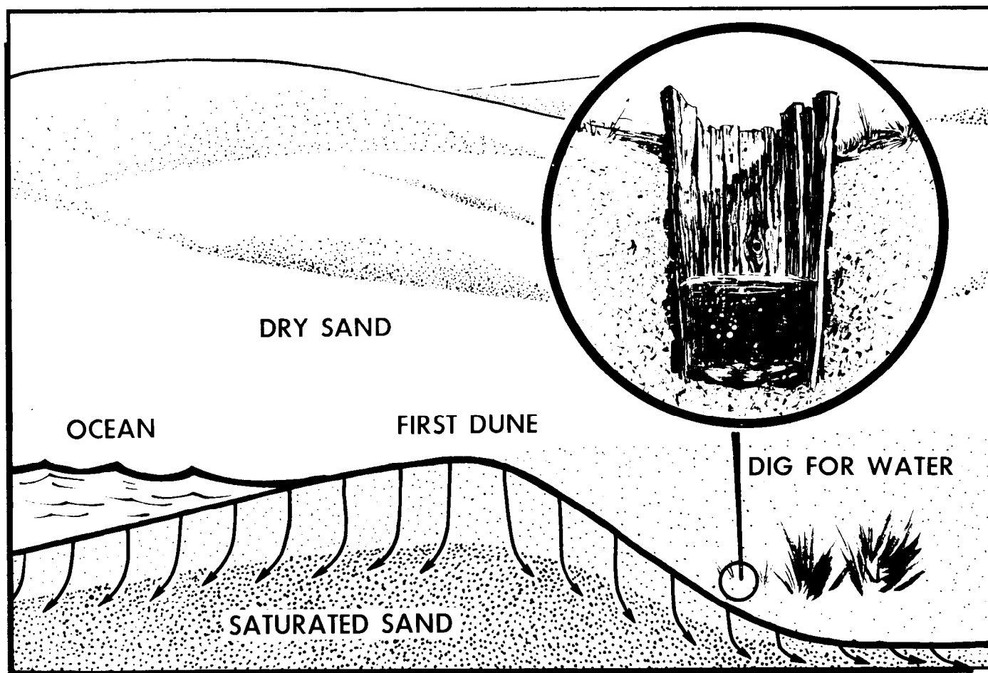
Figure 19-3. Beach Well.
