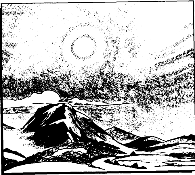
Figure 9-14. Rings Around Moon or Sun.
