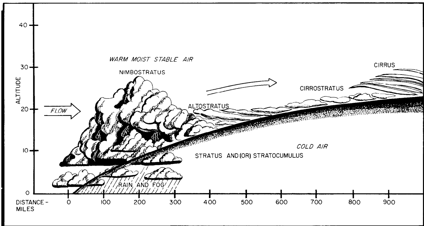
Figure 9-9. Stable Air Warm Front.
