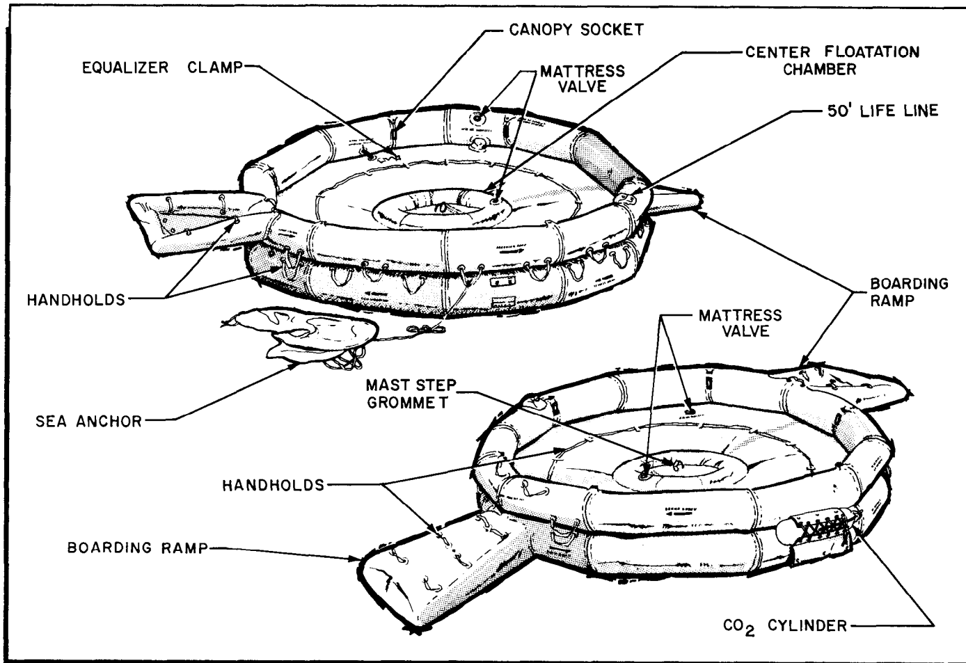
Figure 23-53. 20-Man Raft.
