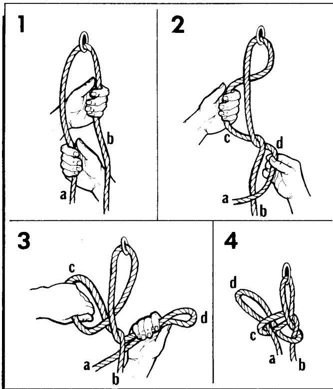
Figure 17-51. Speir Knot.
